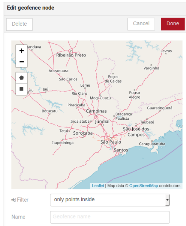
Fig. 11.13: : Geofence configuration
