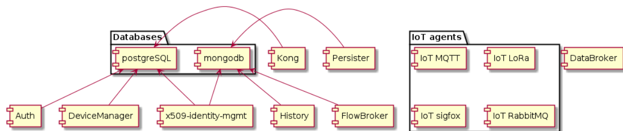
Fig. 5.1: dojoyt components
